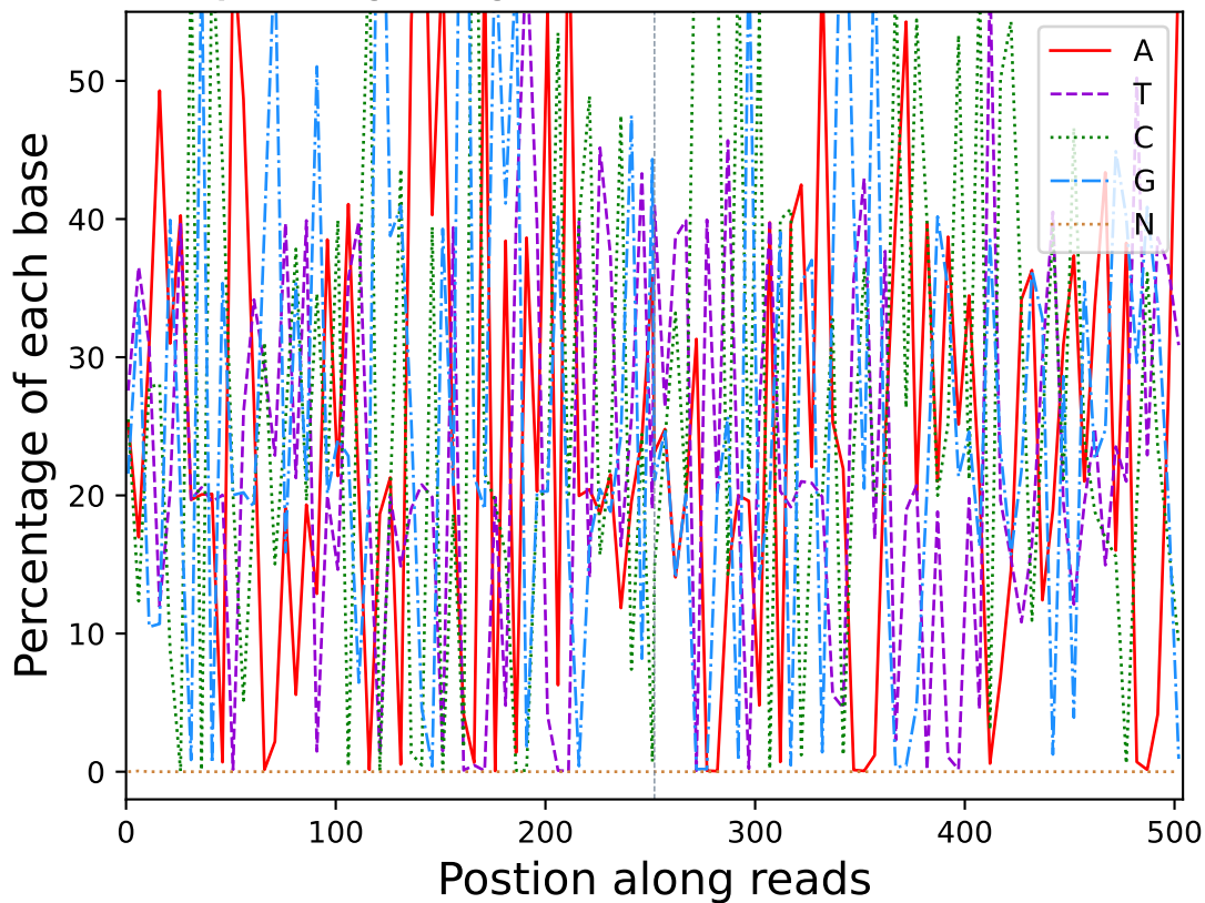
Base percentage along reads (R10127)
